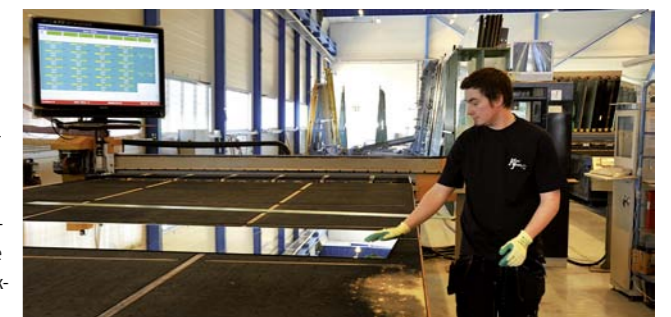
Left: Large glass stock with fully automated loading of the cutting tables. Right: XTV on large screen. The visualisation tool displays cutting pattern and rack allocation – valuable assistance for the employee at the break-out table.
