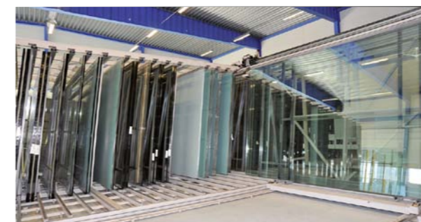
Left: Large glass stock with fully automated loading of the cutting tables. Right: XTV on large screen. The visualisation tool displays cutting pattern and rack allocation – valuable assistance for the employee at the break-out table.
